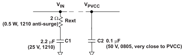
Figure 39. Recommended Input Filter Design
